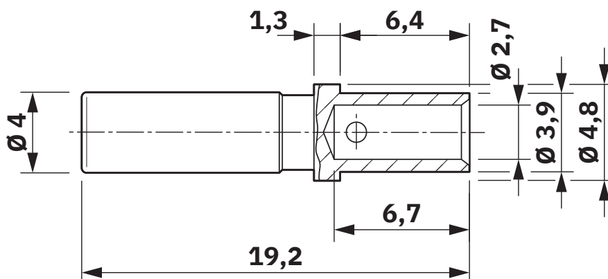
Dimensional drawing
