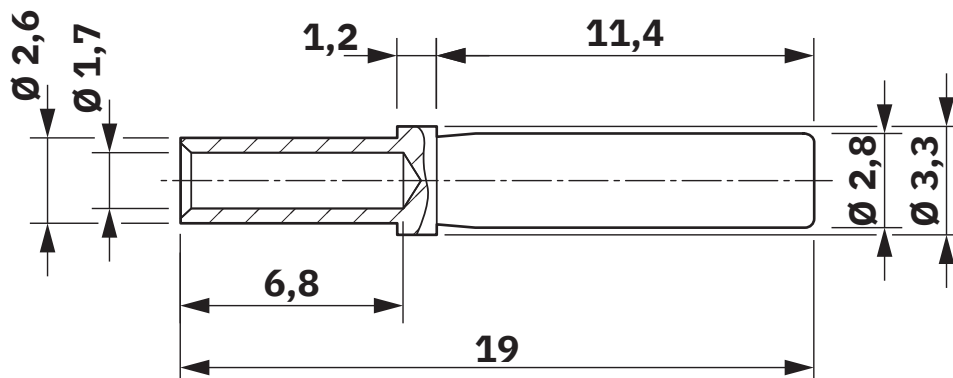
Dimensional drawing
