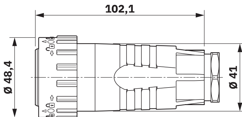
Dimensional drawing
