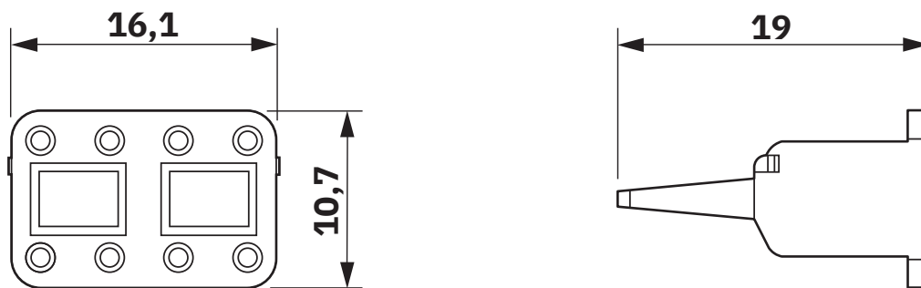
AWM-8S top view and side view
