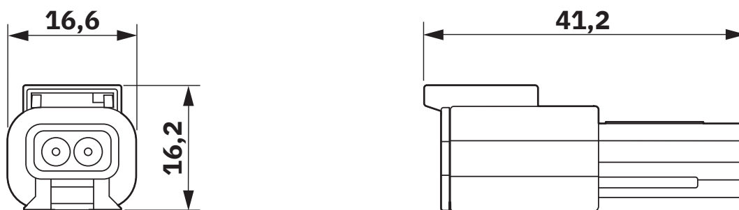
ATM04-2P top view and side view
