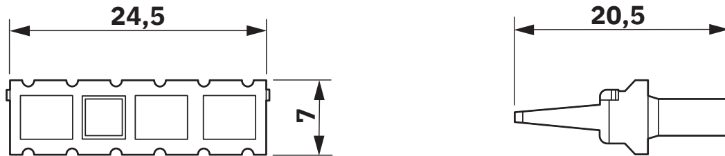
AWM-12P top view and side view
