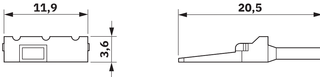
AWM-3P top view and side view
