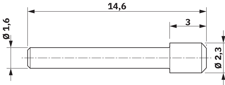
Dimensional drawing
