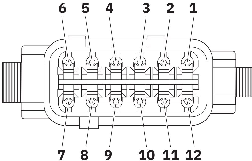
ATM06-12SA pin assignment
