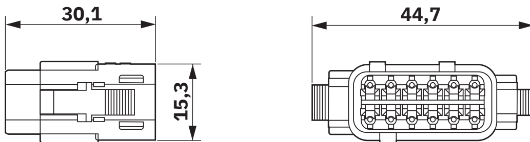
ATM06-12SA top view and side view
