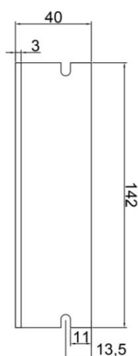
散热机壳尺寸图 ( HEAT SINK DRAWING)
