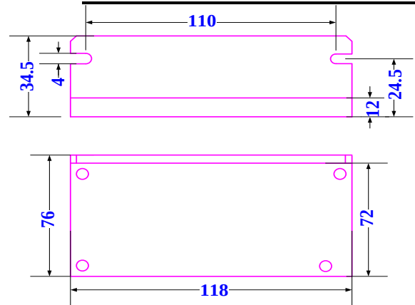
散热机壳尺寸图 (HEAT SINK DRAWING)
