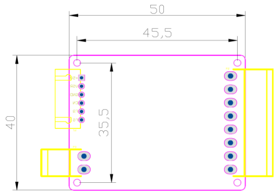
PCB尺寸图 (PCB DRAWING)
