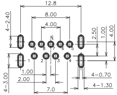
RECOMMENDED PCB LAYOUT(TOP VIEW) GENERAL TOLERANCES:±0.05(T=1.6/1.2)
