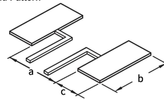
Land Pattern
