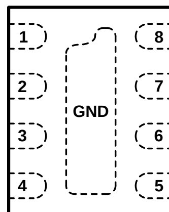
DFN2116P8X (Top View)
