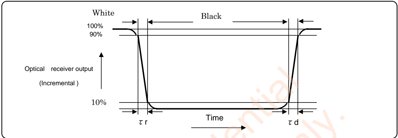
Figure 7-4 Response time
