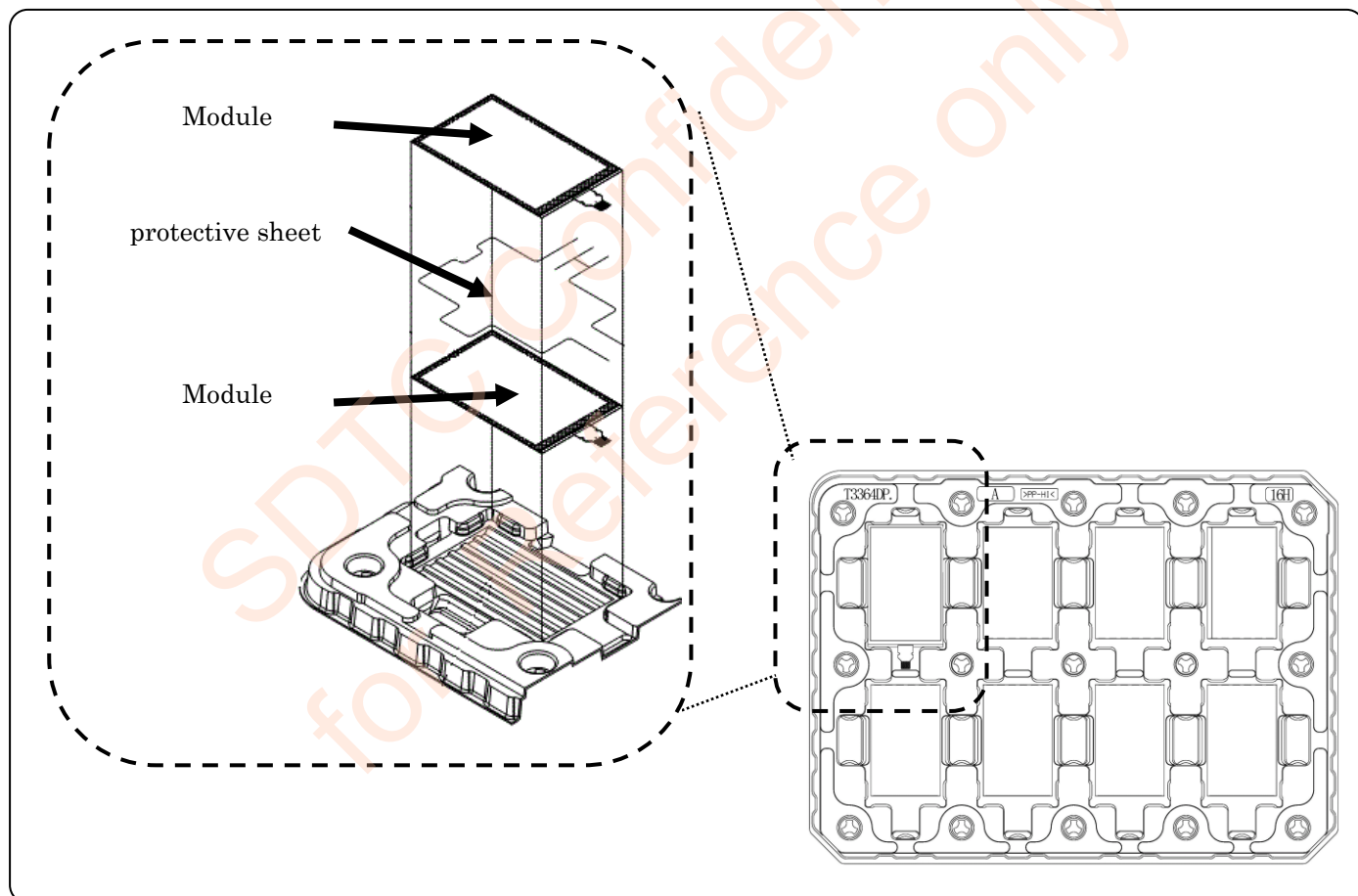
Figure. 12-3-1 Packaging Form 1 ( Tray )
