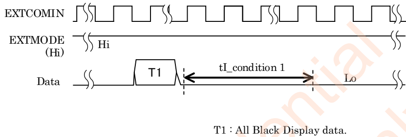
Figure 6-4-1 Current measurement 1
