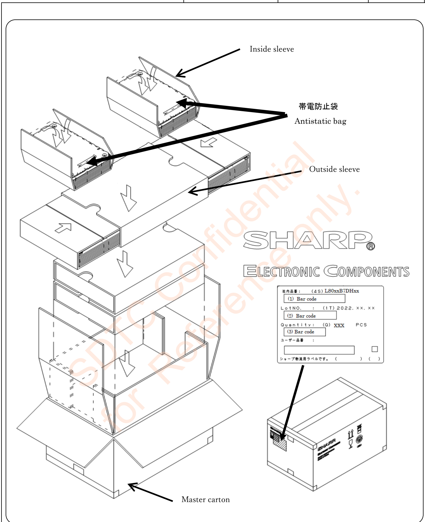
Figure. 12-3-2 Packaging Form 2 (carton)
