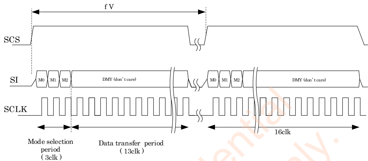
Figure 6-6-3 HOLD mode
