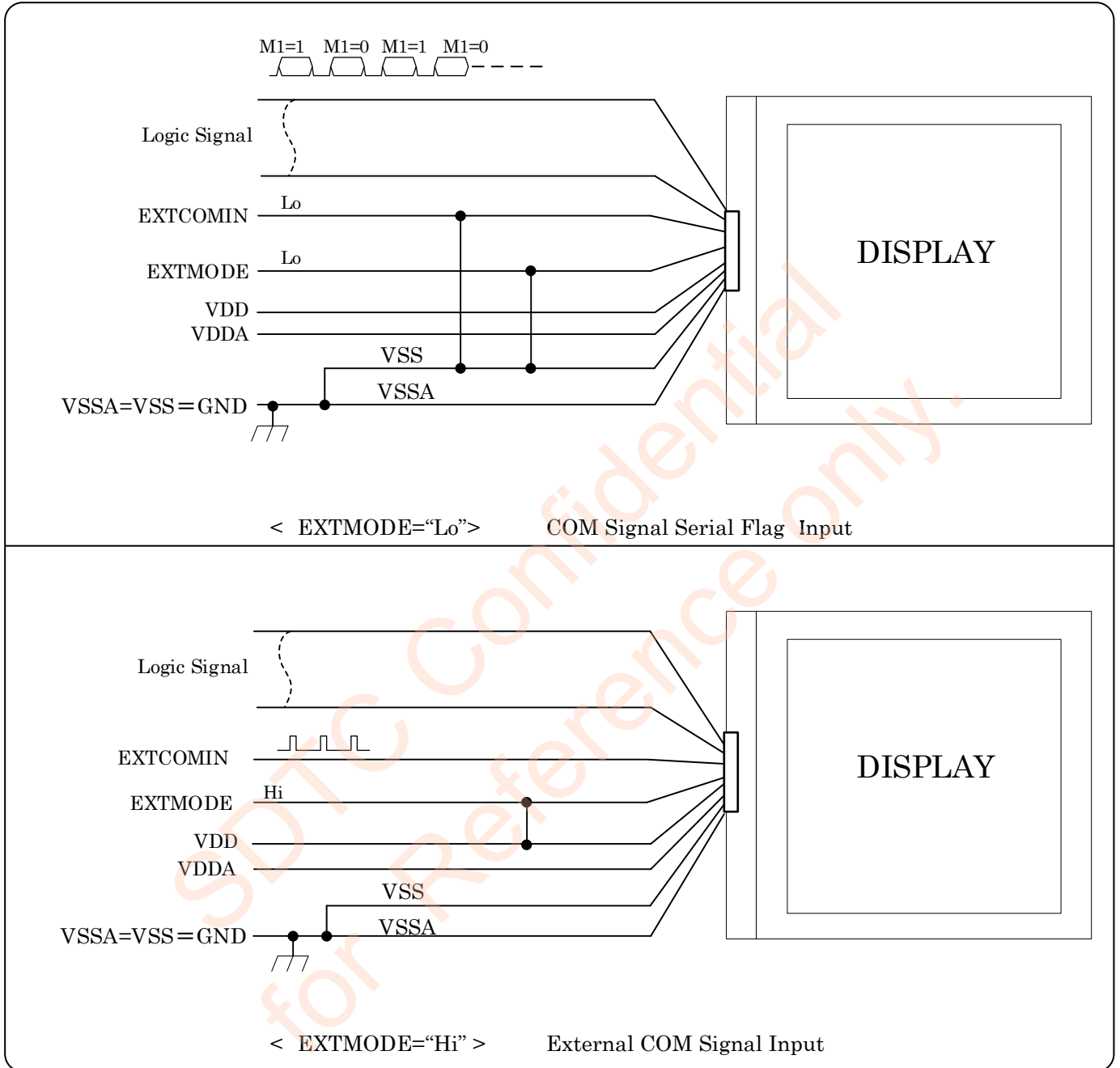
Figure 4-2-1 Recommended circuit
