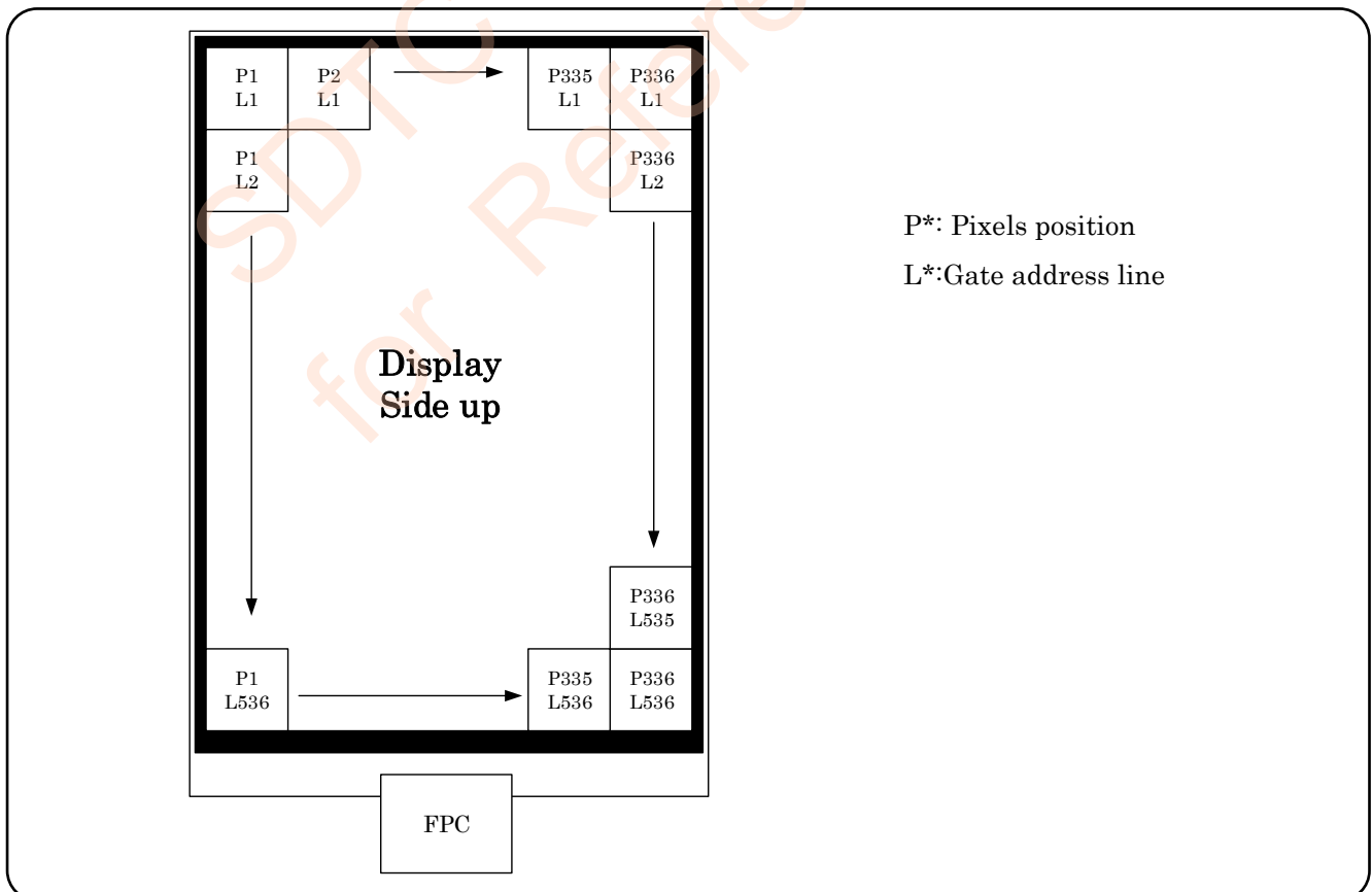
Figure 6-8-1 Data position
