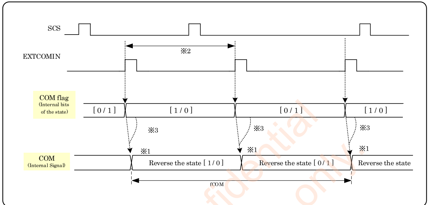
Figure 6-6-7 COM Inversion (EXTMODE=Hi) 2
