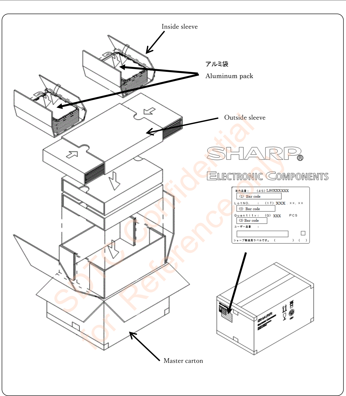
Figure. 12-3-2 Packaging Form 2 (carton) ΔA ΔB
