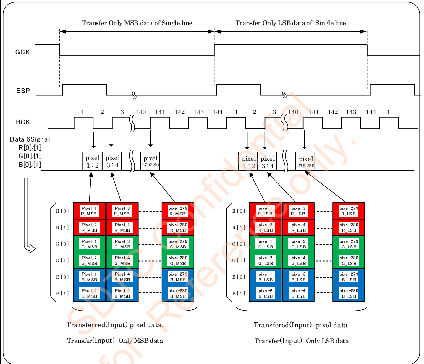
Figure 6-5-2 Horizontal Diagram
