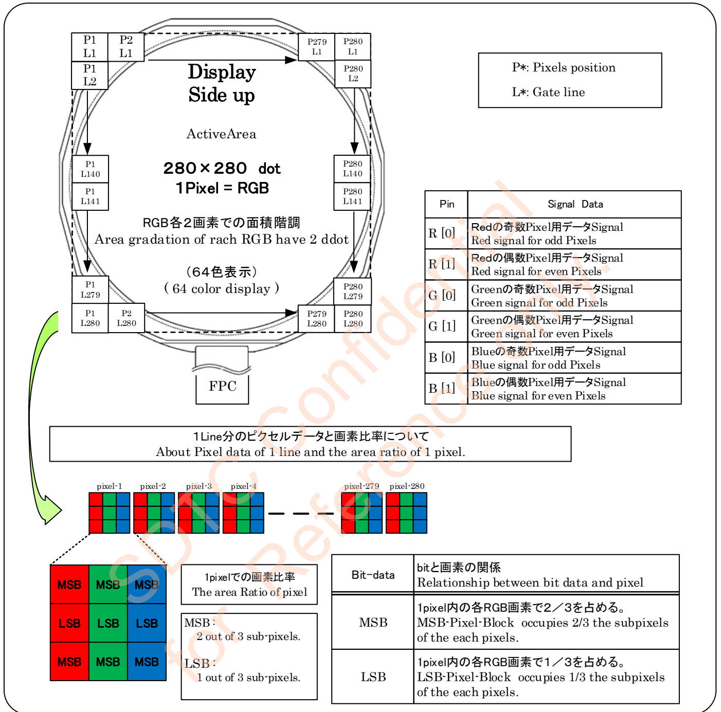
Figure 6-6-1 Data position 1
