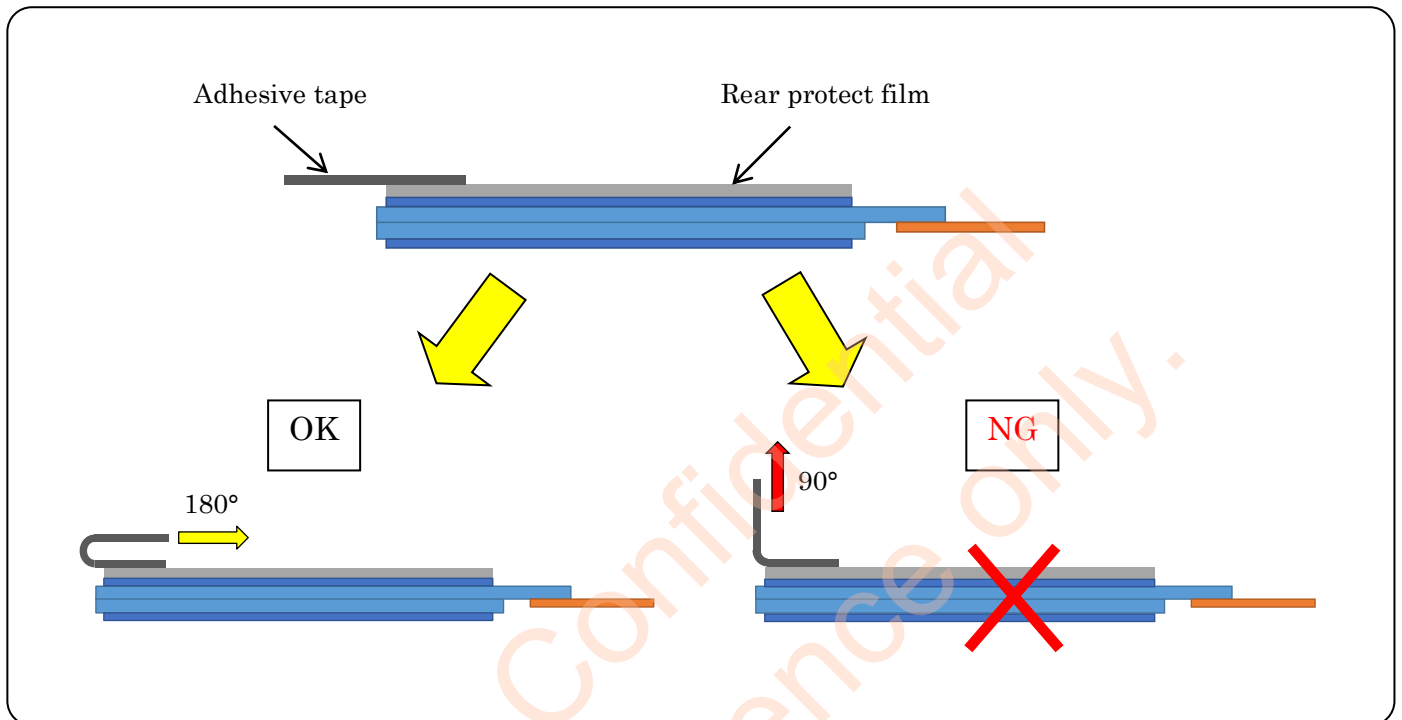
Figure POL-2 Peel angle
