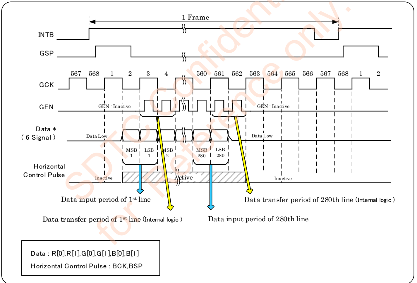
Figure 6-5-1 Vertical Diagram
