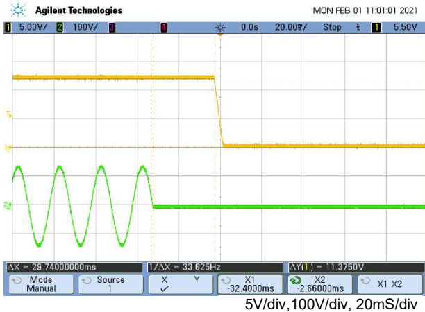
Hold-up time
