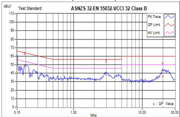
EMI: EN55011 "B" (Conduction)
