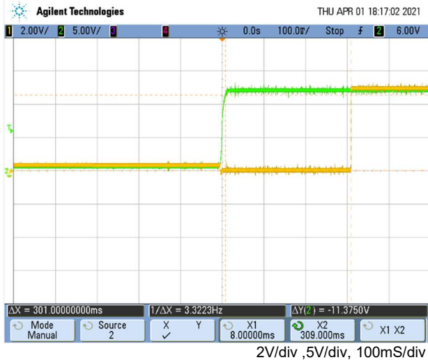
PG(Input voltage: 100Vac)
