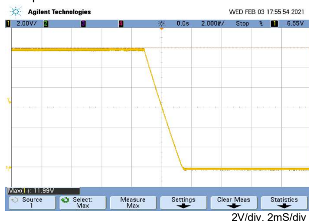
Output turn-off
