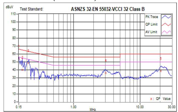
EMI: FCC "B" (Conduction)
