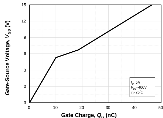
Fig. 18 Typ. Gate Charge at V_{DS}=400\text{V} , I_D=5\text{A}
