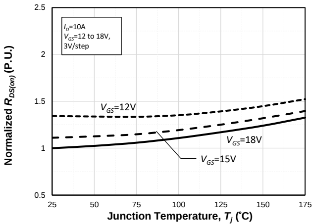
Fig. 6 Normalized R_{DS(on)} vs. T_j with Various V_{GS}
