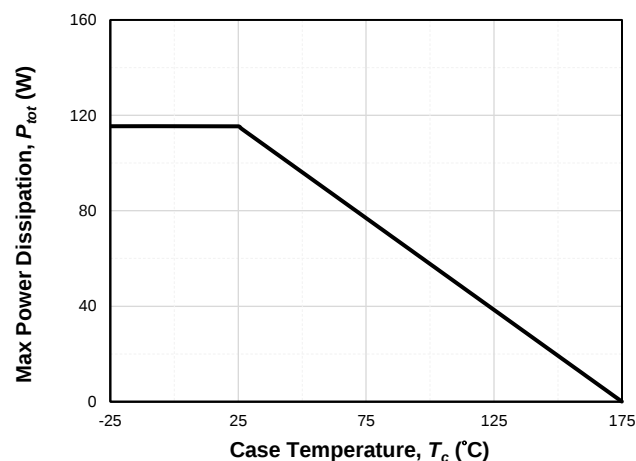
Fig. 11 Power Dissipation at V_{GS} = 18\text{V} , T_J \leq 175^\circ\text{C}
