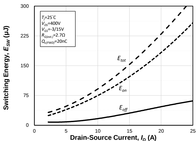
Fig. 24 Typ. Switching Energy vs. I_D
