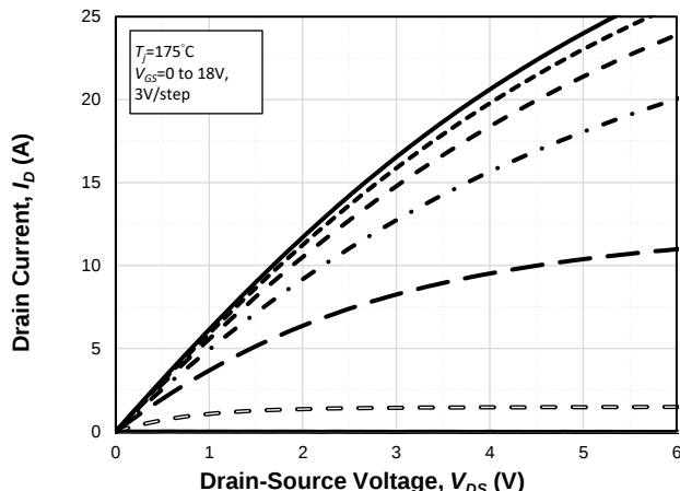
Fig. 2 Typical Output Characteristics at T_j = 175^\circ\text{C}
