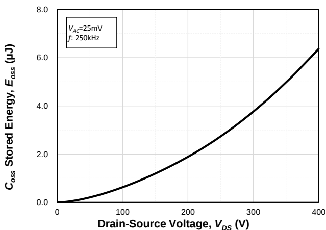
Fig. 17 Typ. C_{oss} Stored Energy at f_{sw}=250\text{kHz}
