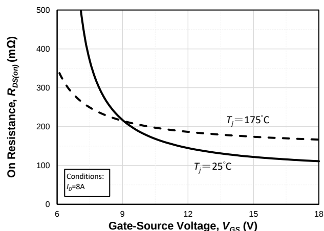
Fig. 7 Typ. R_{DS(on)} vs. V_{GS} with Various T_J
