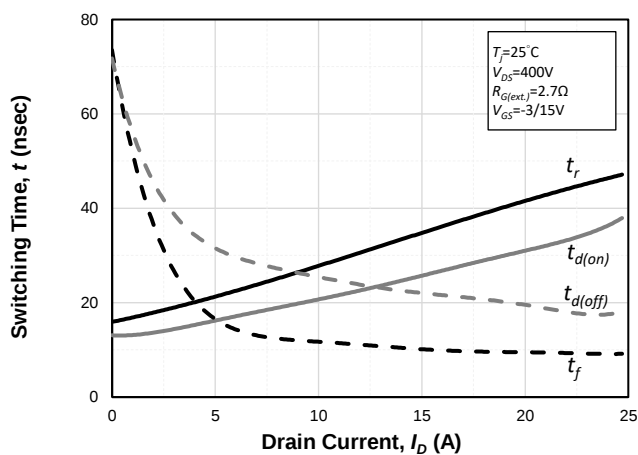
Fig. 22 Typ. Switching Time vs. I_D
