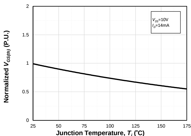
Fig. 8 Normalized V_{th} vs. T_J
