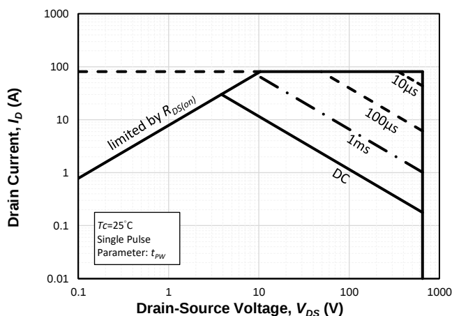
Fig. 12 Safe Operating Area at T_c = 25^\circ\text{C}
