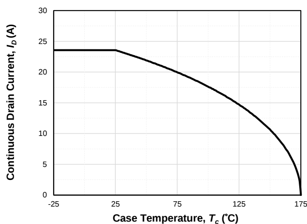
Fig. 10 Continuous I_D De-rating at V_{GS} = 18\text{V} , T_J \leq 175^\circ\text{C}
