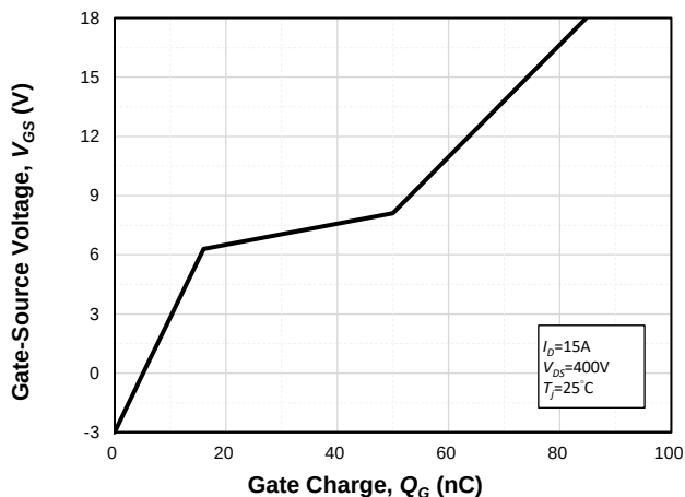
Fig. 19 Typ. Gate Charge at V_{DS}=400V , I_D=15A
