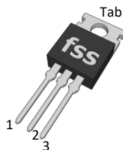
TO-220-3L
