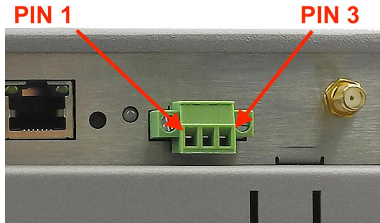
Power Input
