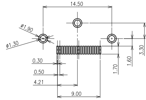
PCB LAYOUT(TOP VIEW) (T=1.60mm)
