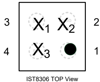
IST8306 TOP View
