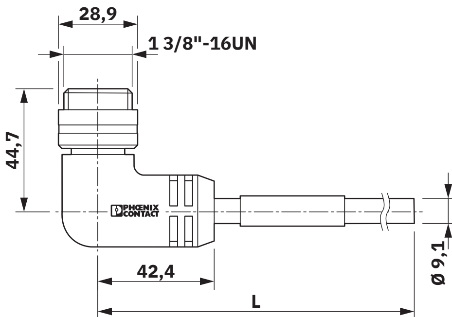
Dimensional drawing
