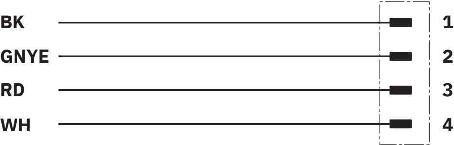
Circuit diagram
