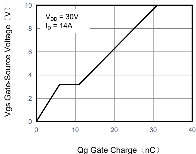
Figure 4. Gate Charge
