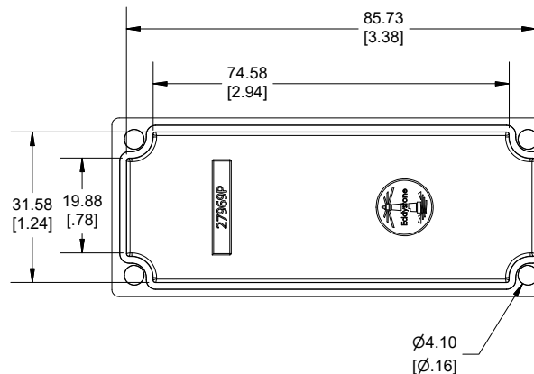
INSIDE LID VIEW
