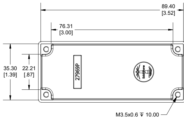
INSIDE BOX VIEW
