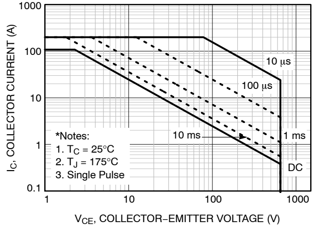
Figure 8. SOA Characteristics
