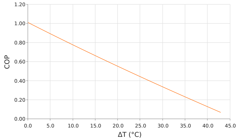
Coefficient of Performance (COP = Qc/Pin) Voperating = 24.02 Volts | Ioperating = 10.81 Amps
