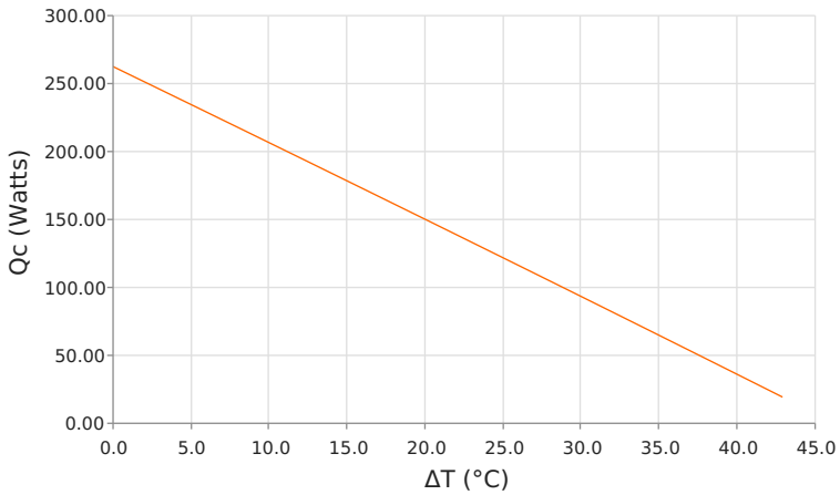
Heat Pumped at Cold Side (Qc) Voperating = 24.02 Volts | Ioperating = 10.81 Amps
