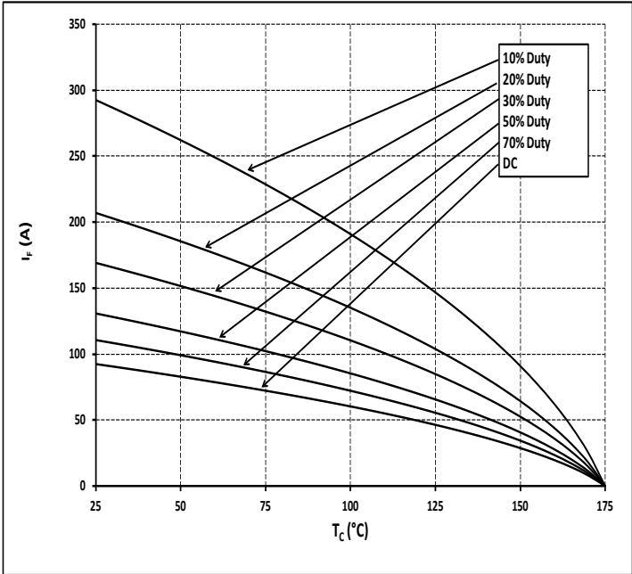
Figure 3 Current Derating
