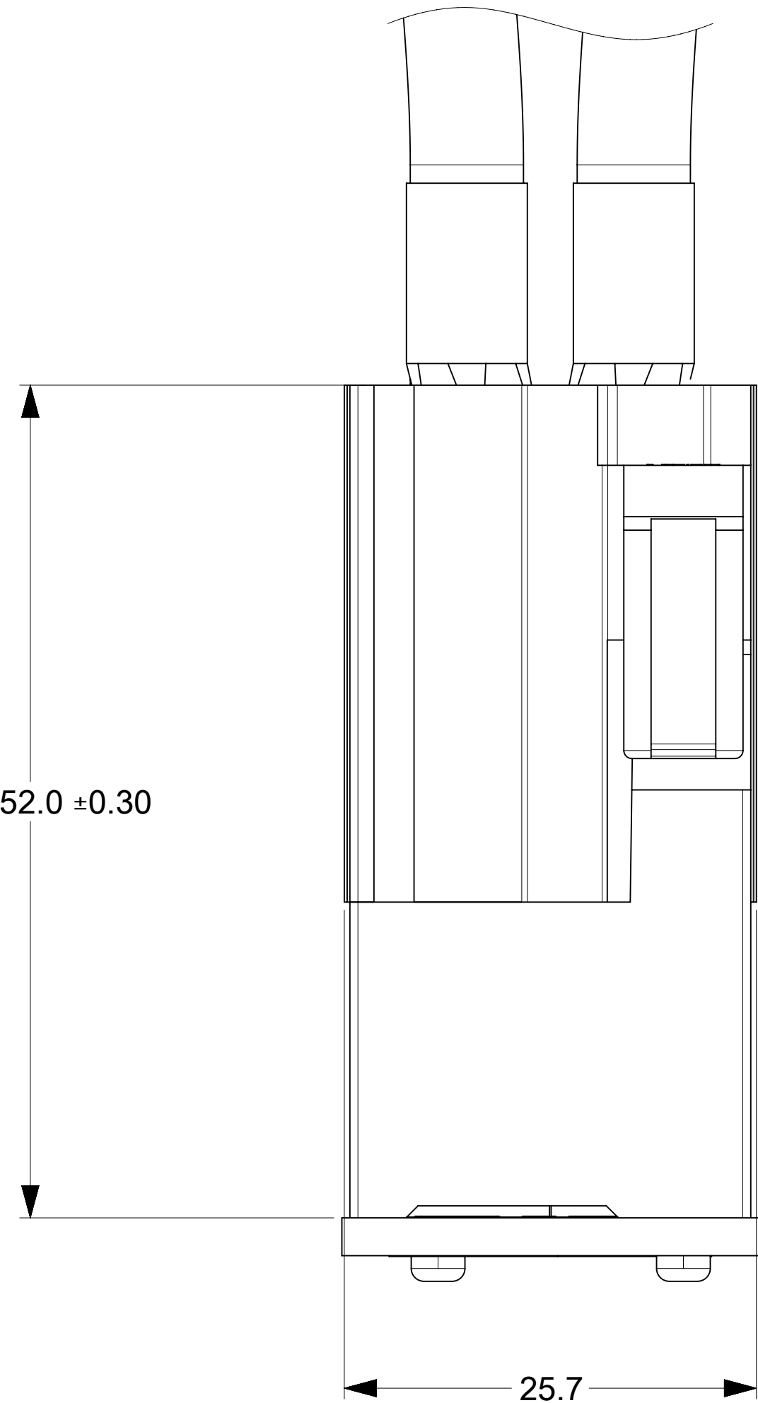
MATED WITH VERTICAL RECEPTACLE
