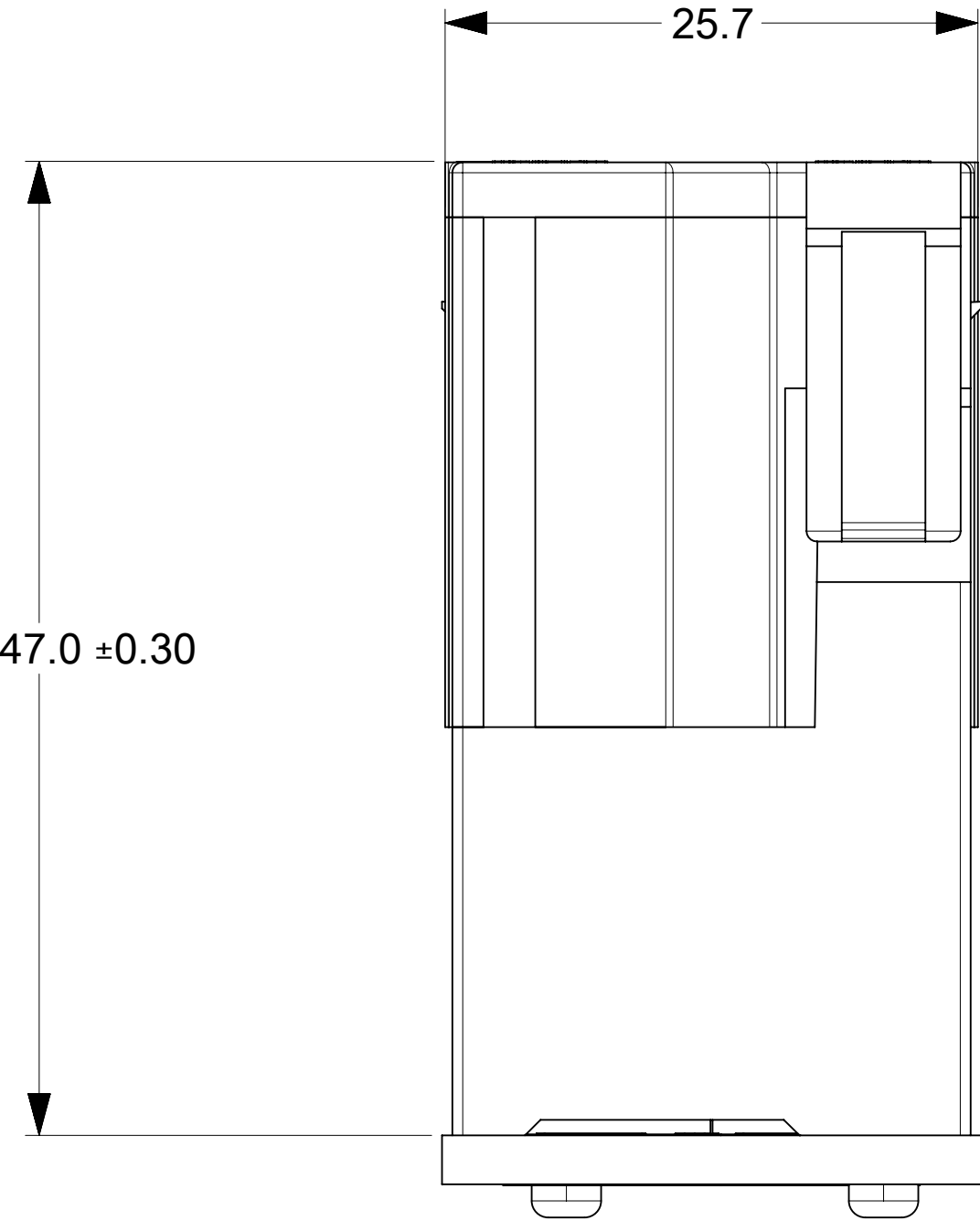
MATED WITH RIGHT ANGLE RECEPTACLE
