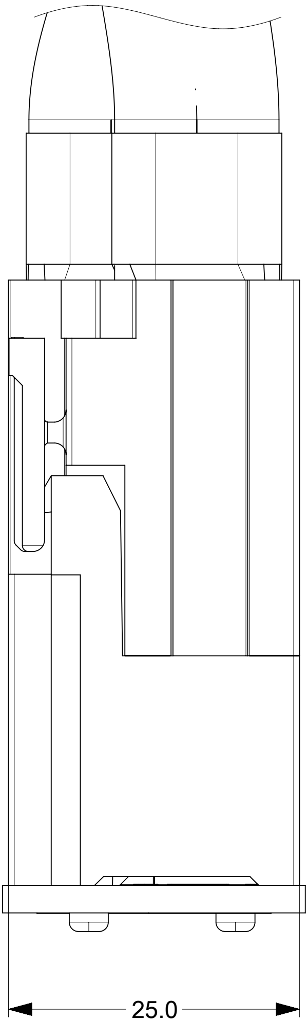
MATED WITH VERTICAL RECEPTACLE
