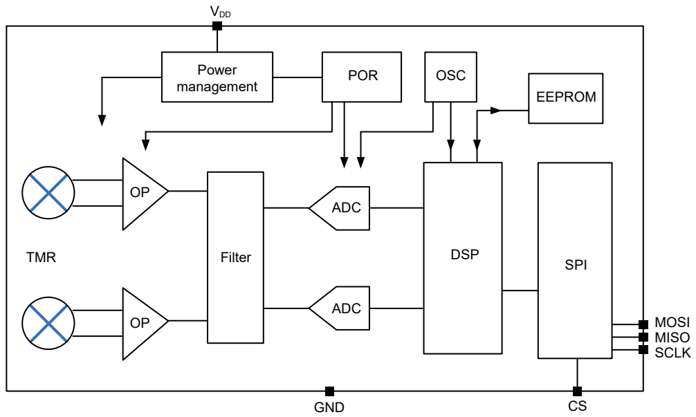
Figure 2. TMR3109 functional block diagram
