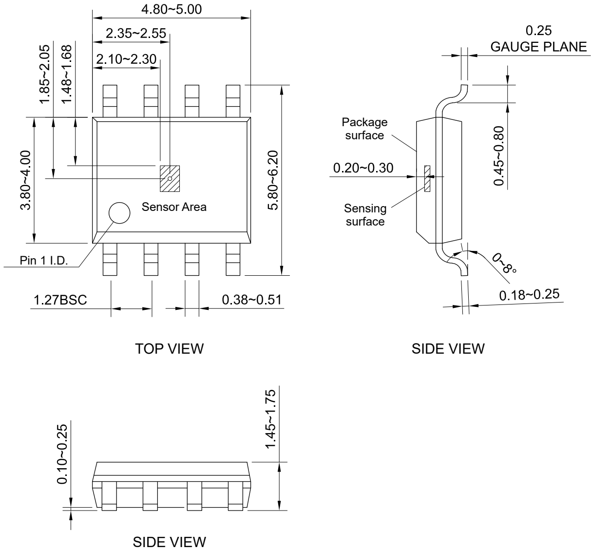
Figure 17. Package outline of SOP8 (unit: mm)
