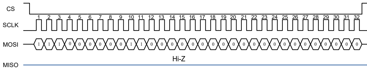
Figure 9. User mode to normal mode change sequence diagram
