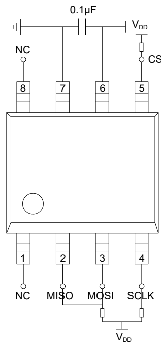
Figure 15. Schematic of 3-wire SPI circuit
