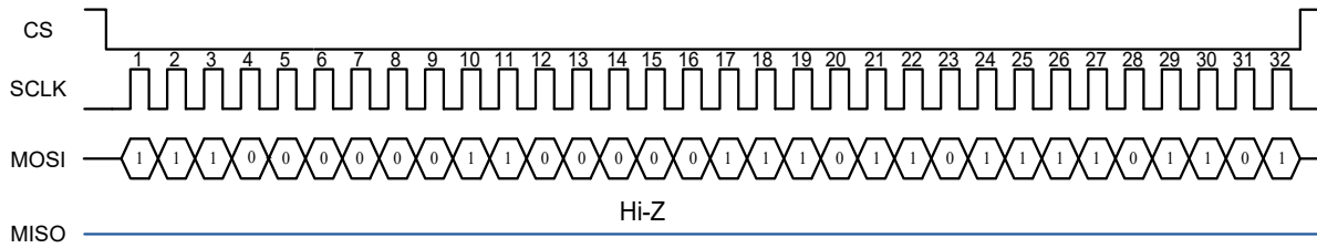
Figure 8. Normal mode to user mode change sequence diagram
