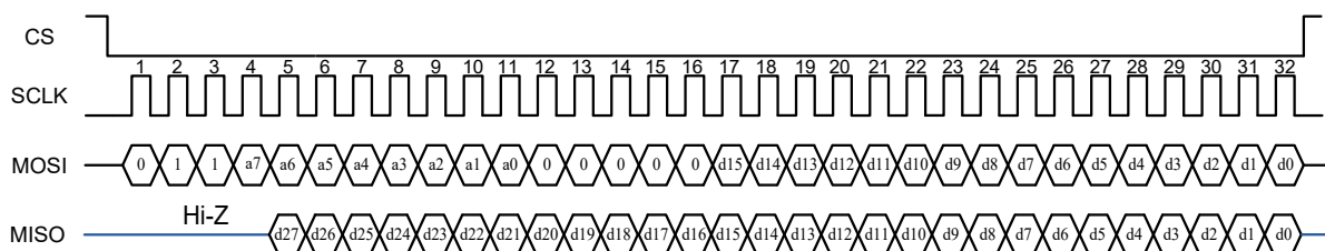
Figure 10. SPI read angle sequence diagram
