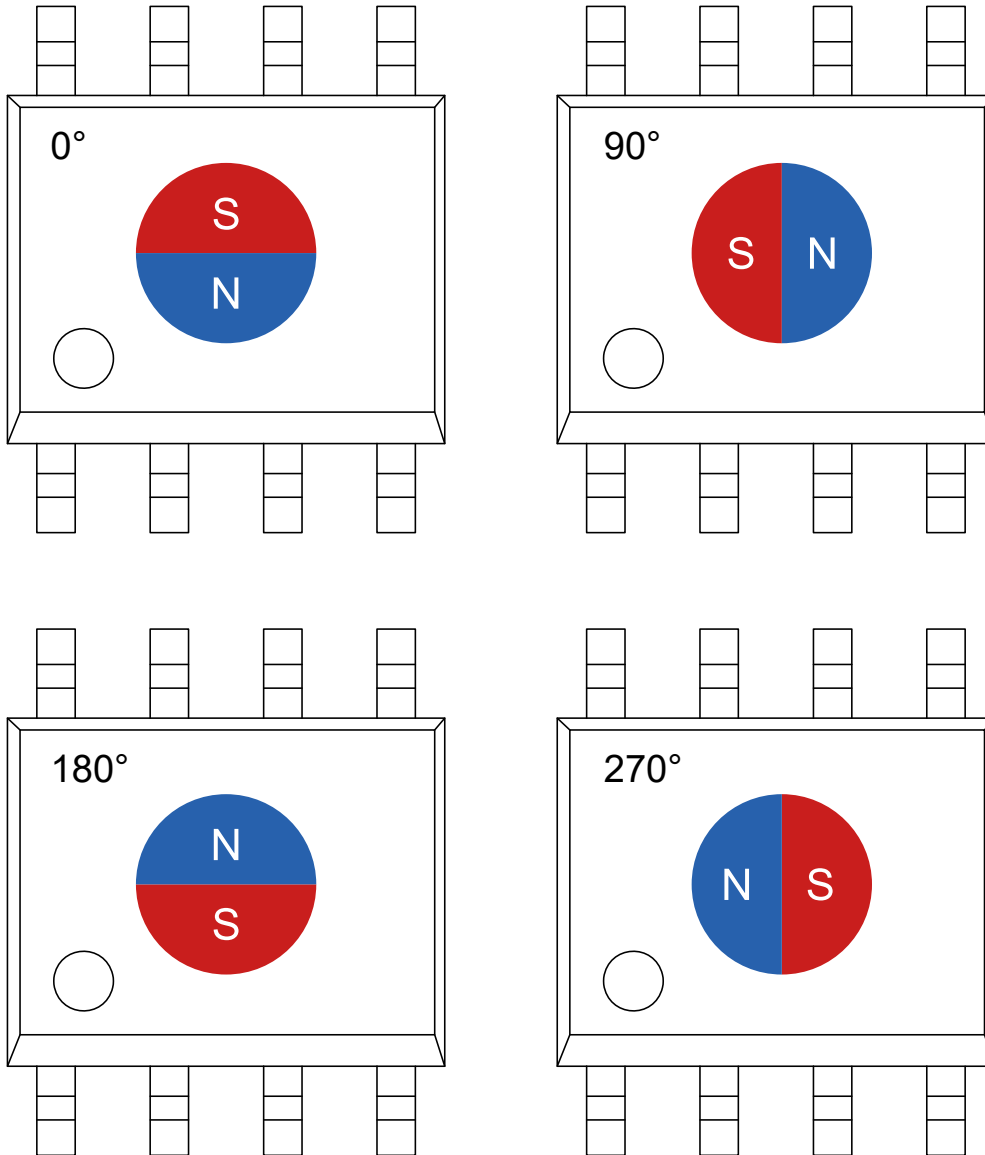
Figure 16. Definition of the magnetic field orientation measured by TMR3109
