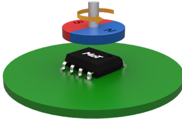
Figure 12. Self-calibration schematic
