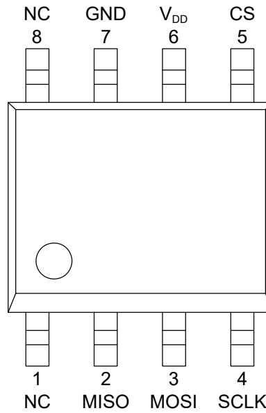
Figure 1. Pin configuration (SOP8)
