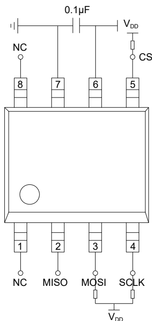
Figure 14. Schematic of 4-wire SPI circuit
