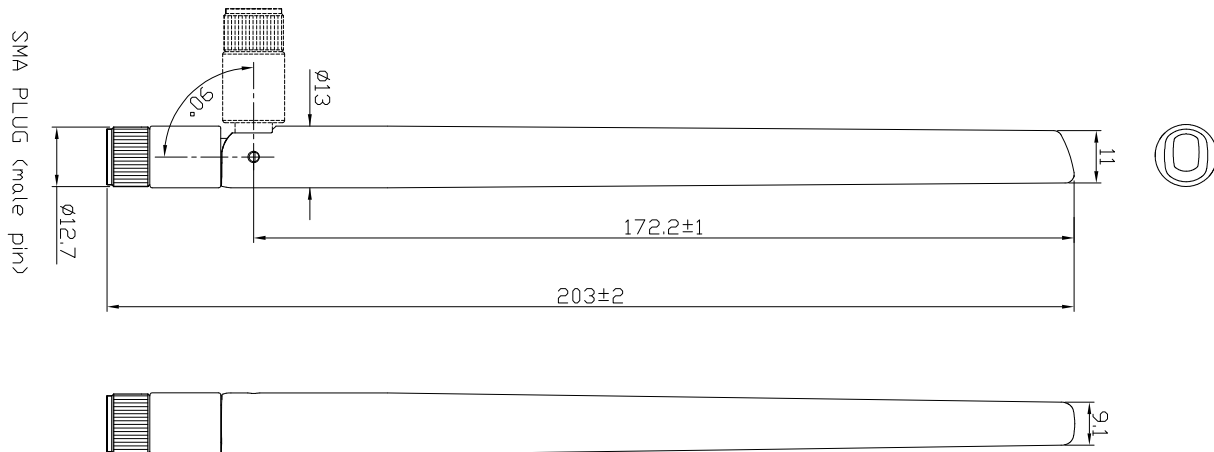
Figure 2. Antenna Dimensions
