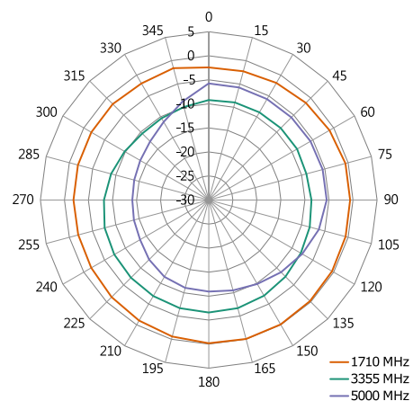
XY-Plane Gain
