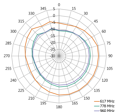
XY-Plane Gain
