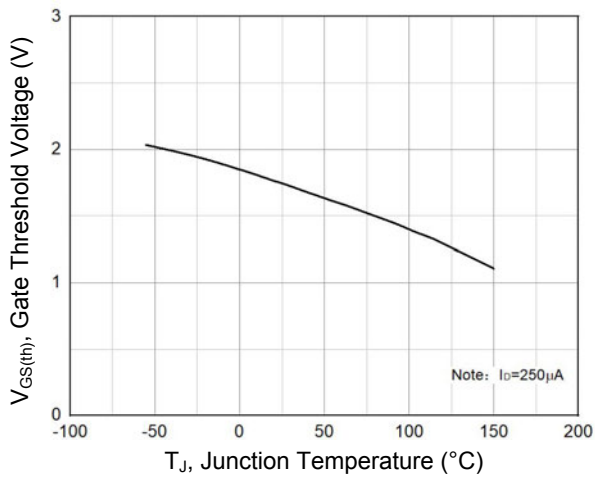
Figure 9. Gate Threshold Voltage vs. T J
