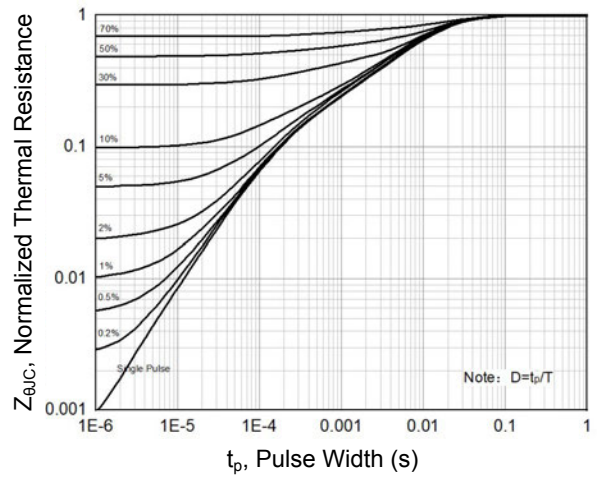
Figure 10. Transient Thermal Impedance vs. t p
