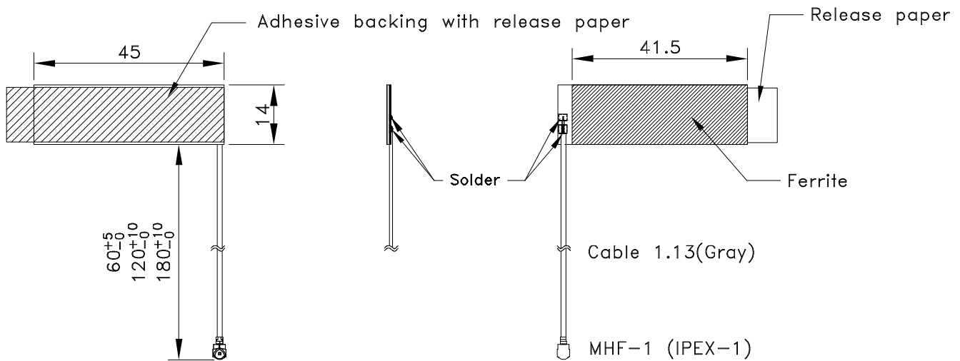
Figure 2. Antenna Dimensions
