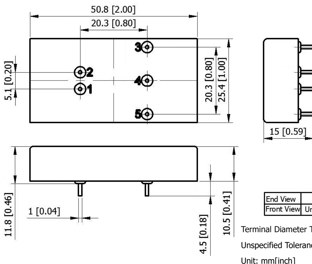
Figure 6. Outline Dimensions
