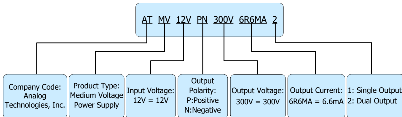
Naming Principle of ATMV12VPN300V6R6MA2
