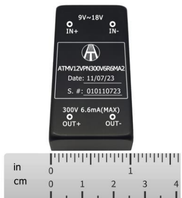
Figure 1. Top View of ATMV12VPN300V6R6MA2
