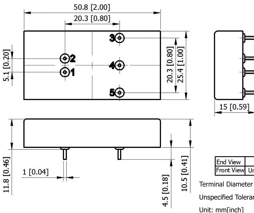
Figure 6. Outline Dimensions
