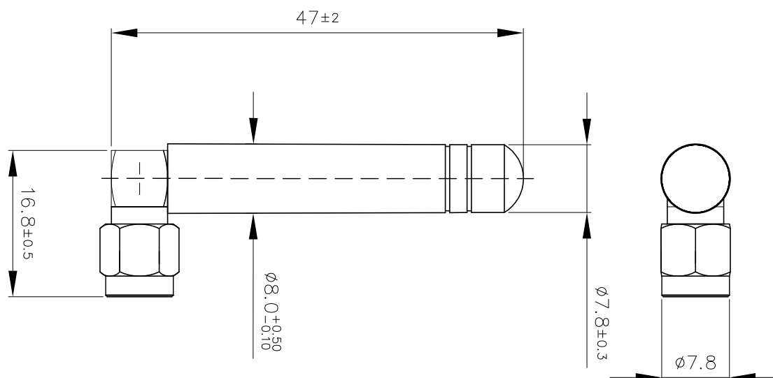
Figure 2. Antenna Dimensions
