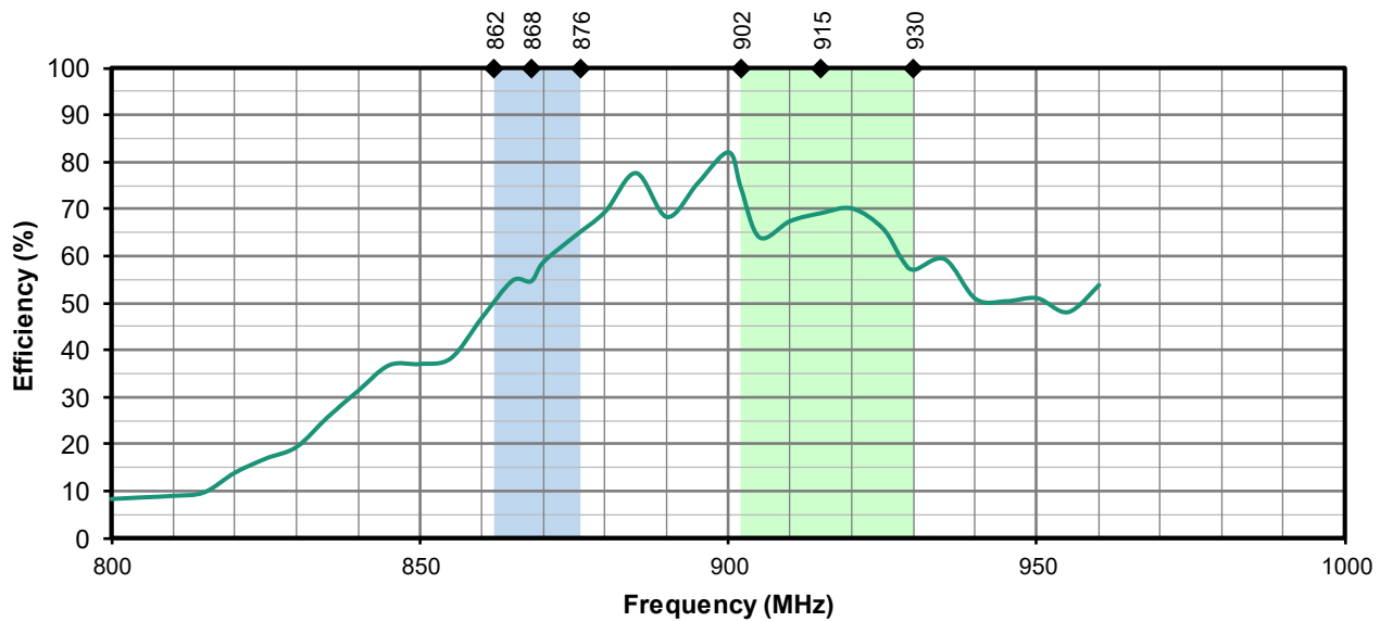
Figure 8. Antenna Efficiency
