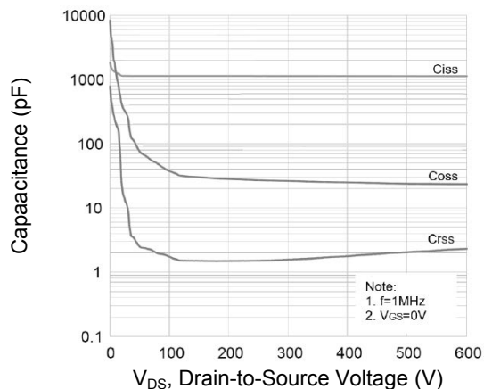
Figure 7. Capacitance Characteristics
