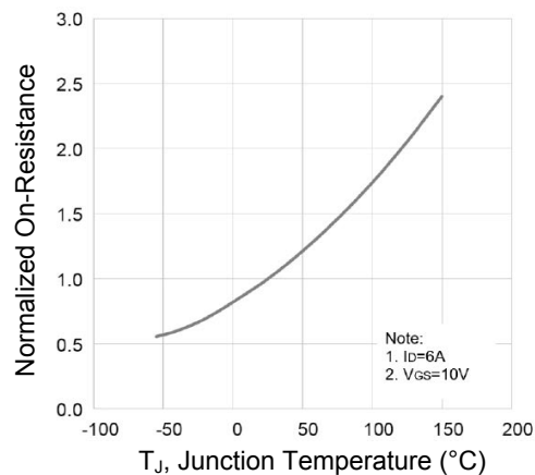
Figure 8. Normalized R_{DS(ON)} vs. T_J
