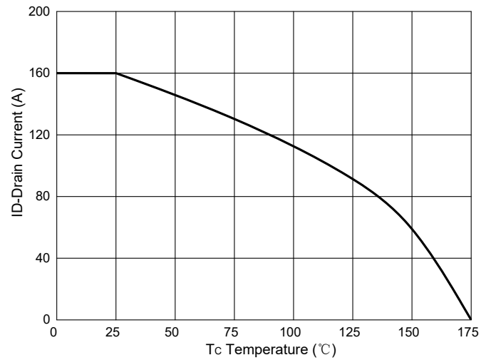
Fig. 10 - Drain Current
