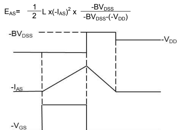
Figure 8. EAS Waveform
