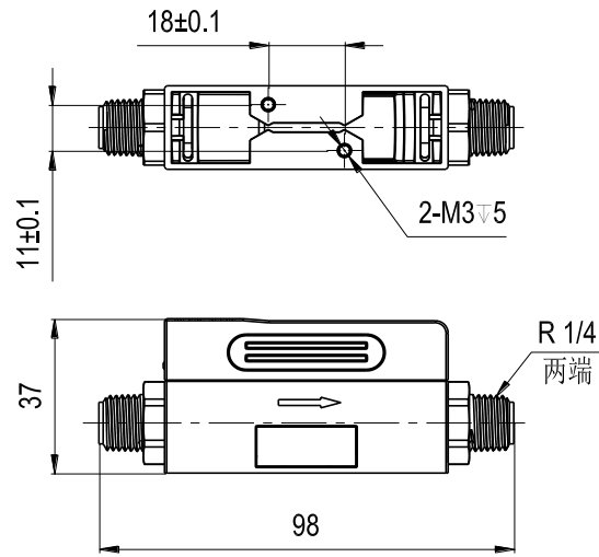
Figure 4: PFLOW3000 dimensions with BSPT (R1/4") connectors. All units are in mm
