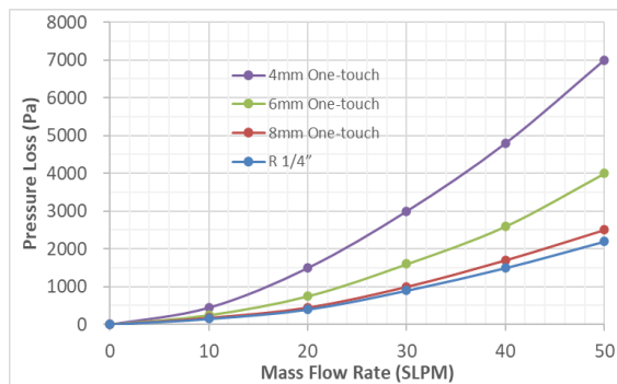
Figure 3: PFLOW3008-30/40/50 pressure loss
