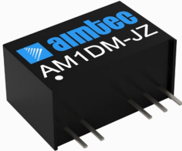
SIP7 Package
