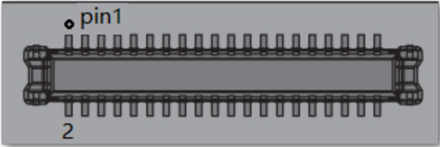
Figure 7: WisBlock Core module 40-pin connector
