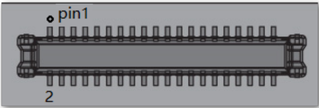
Figure 6: WisBlock Core module 40-pin connector
