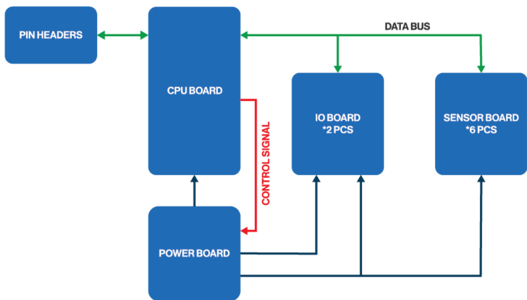
Figure 2: RAK19011 WisBlock Base block diagram
