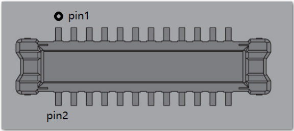
Figure 8: WisBlock 24-pin module connector
