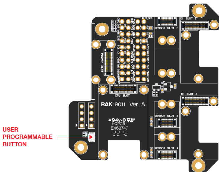
Figure 3: RAK19011 part label
