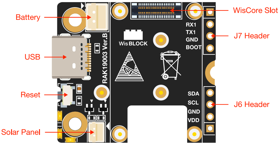
Figure 3: RAK19003 Top View Components
