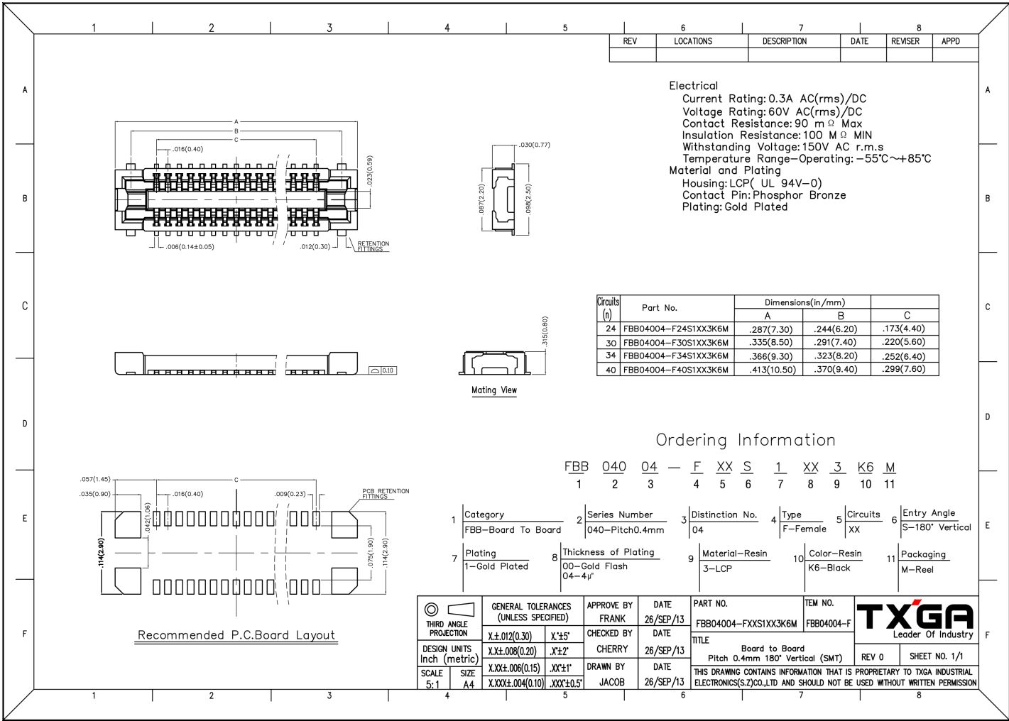
Figure 13: WisConnector PCB Footprint and Recommendations
