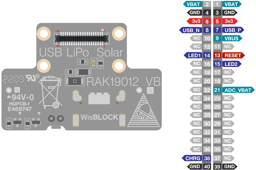
Figure 5: RAK19012 pinout diagram
