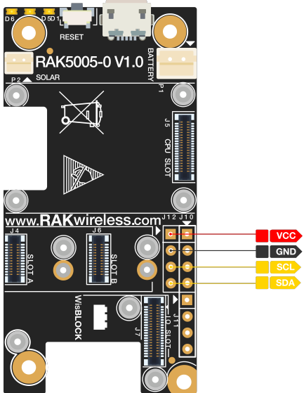
Figure 1: I2C pin header in the RAK5005-O
