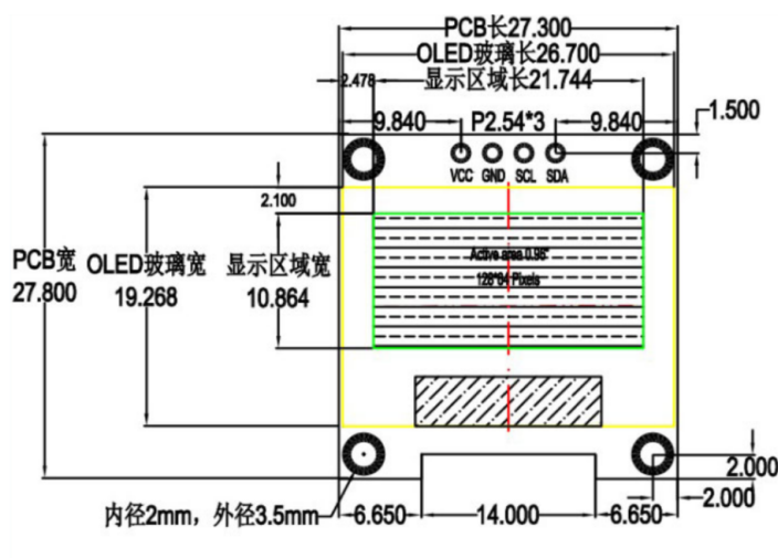
Figure 3: Mechanical Dimensions
