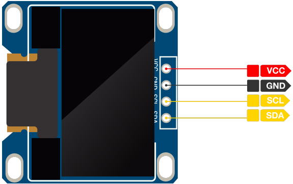
Figure 2: RAK1921 Pin Definition
