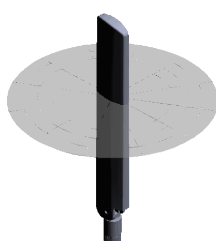
XY-Plane Gain
