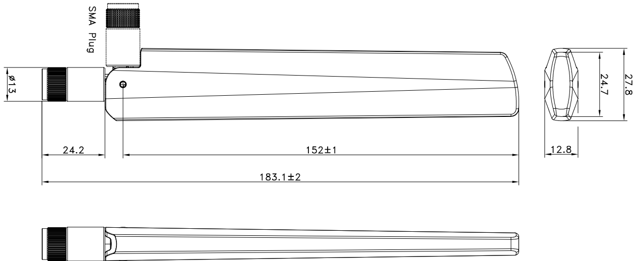
Figure 2. Antenna Dimensions
