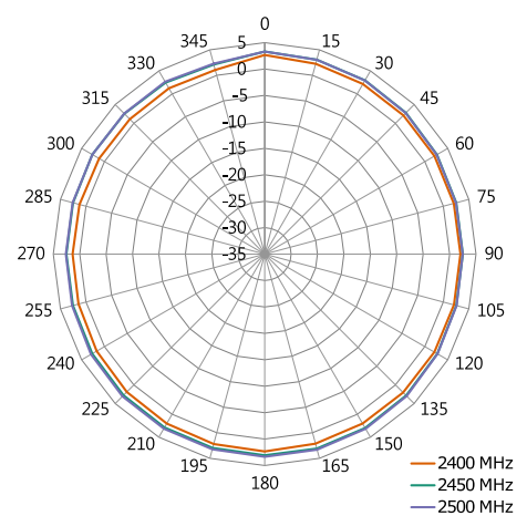
XY-Plane Gain
