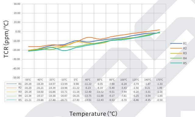
TCR Test Curve - SEWF3951 0.4mΩ
